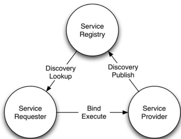
Figure 1: Service-Oriented Architecture
