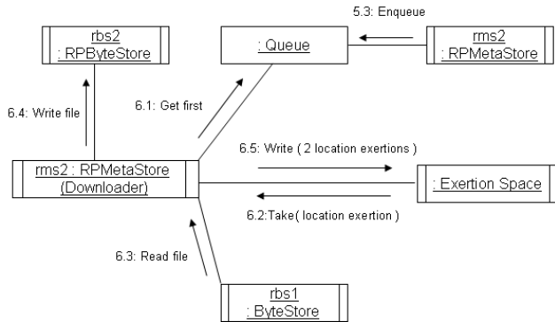
Figure 6: The Processing Update Use Case
