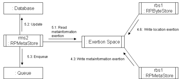
Figure 5: The Scheduling Update Use Case
