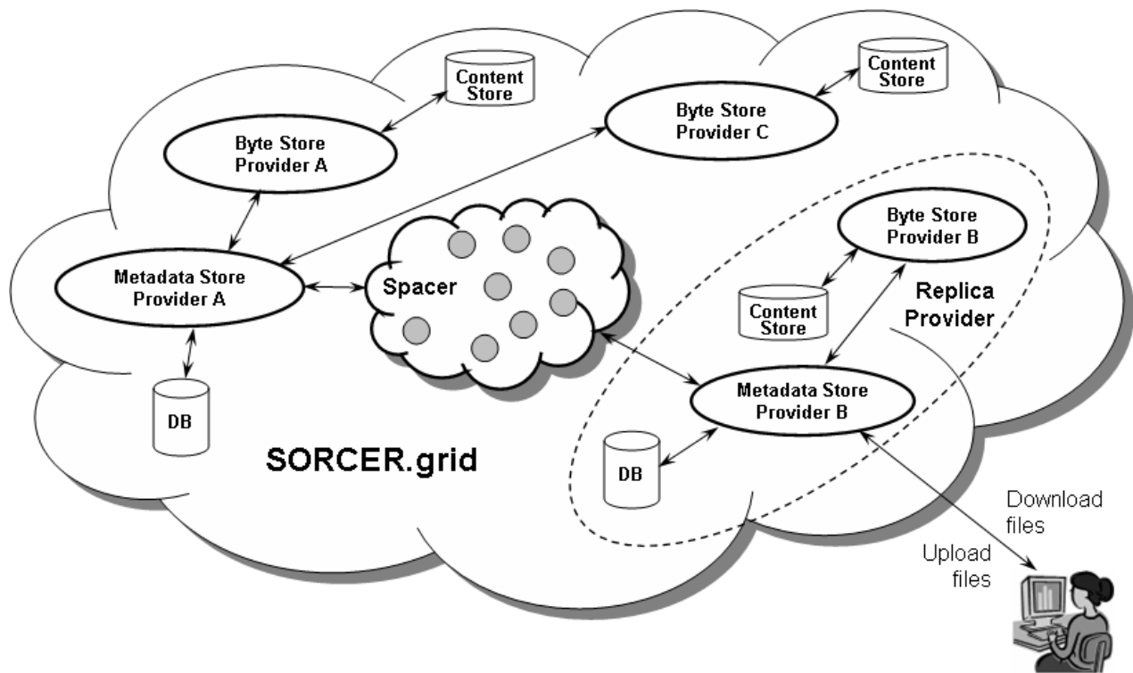
Figure 2: Overview of basic components and the data flow in the replication federation. The federation components are marked by bold outlines.
