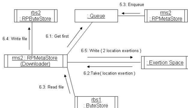
Figure 7: The Reading File Use Case
