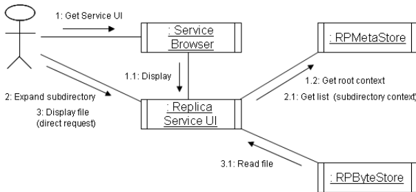
Figure 3: The Browsing Files Use Case
